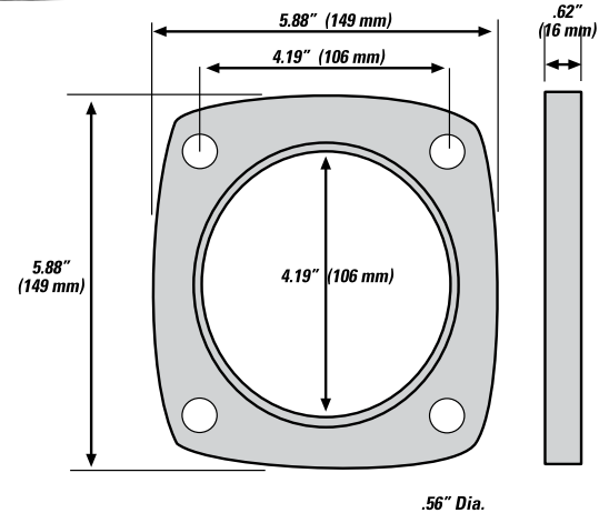
Manifold Flange Part Number P206616
